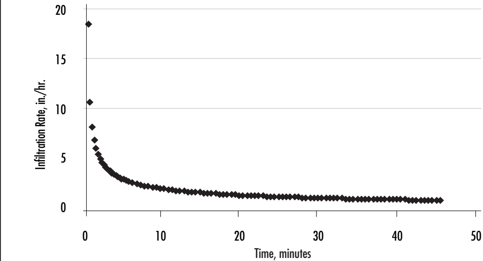
TYPICAL INFILTRATION RATE CURVE
