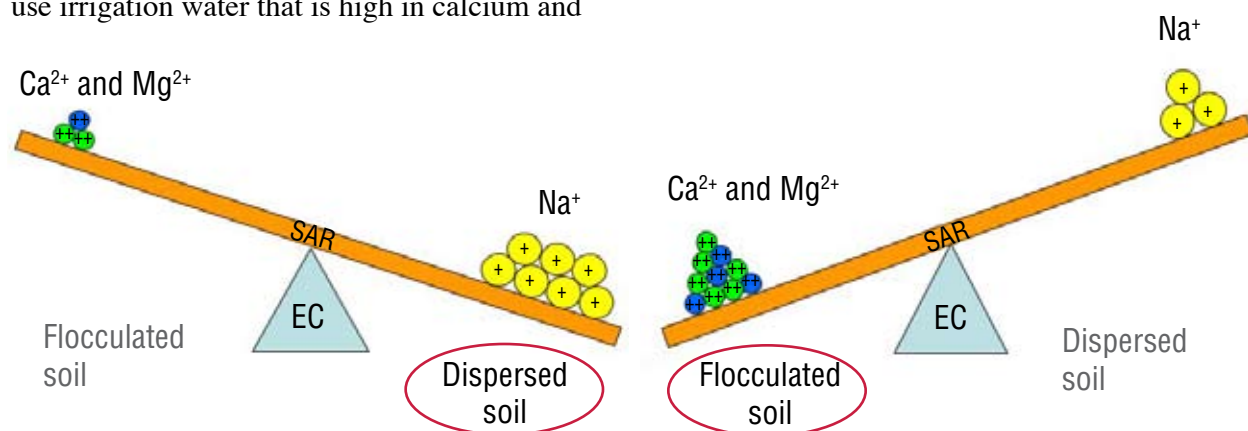
Figure 6.—The “teeter-totter” shows how soil structure (dispersed versus flocculated) depends on SAR (balance between \text{Ca}^{2+} , \text{Mg}^{2+} , and \text{Na}^+ ) and soluble salts (EC) in soil. Soil particles disperse (left) when (\text{Ca}^{2+} + \text{Mg}^{2+}) is decreased relative to \text{Na}^+ (SAR is increased). Soil particles flocculate (right) when (\text{Ca}^{2+} + \text{Mg}^{2+}) is increased relative to \text{Na}^+ (SAR is decreased).
